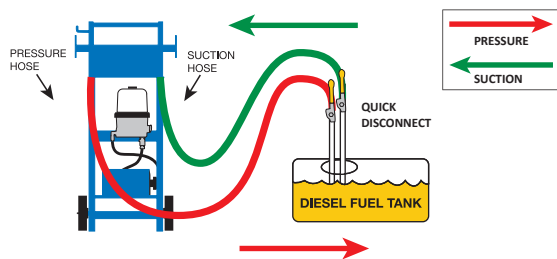
SWEEPING FUEL TANKS
