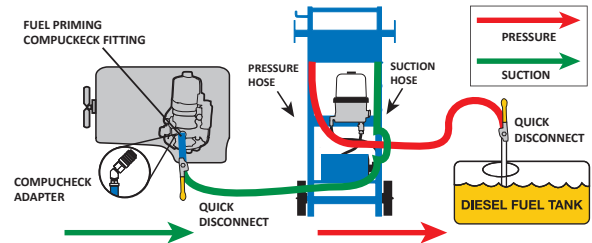
REMOVING FUEL
